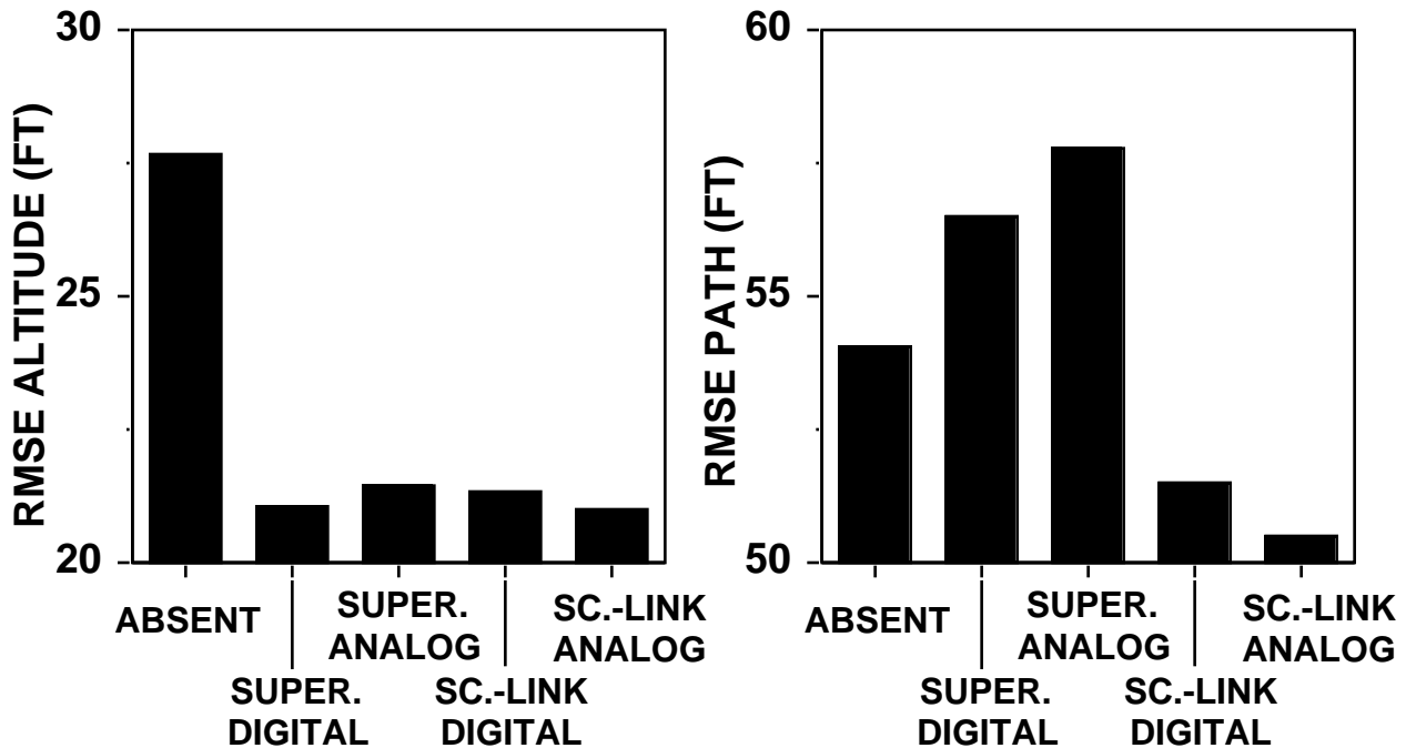
Figure 6. Results of experimental test: Effects of HUD altitude symbology absence, superimposed digital symbology, superimposed analog clock symbology, scene-linked digital symbology and scene-linked analog clock symbology on RMSE Altitude (left) and RMSE Path right).
